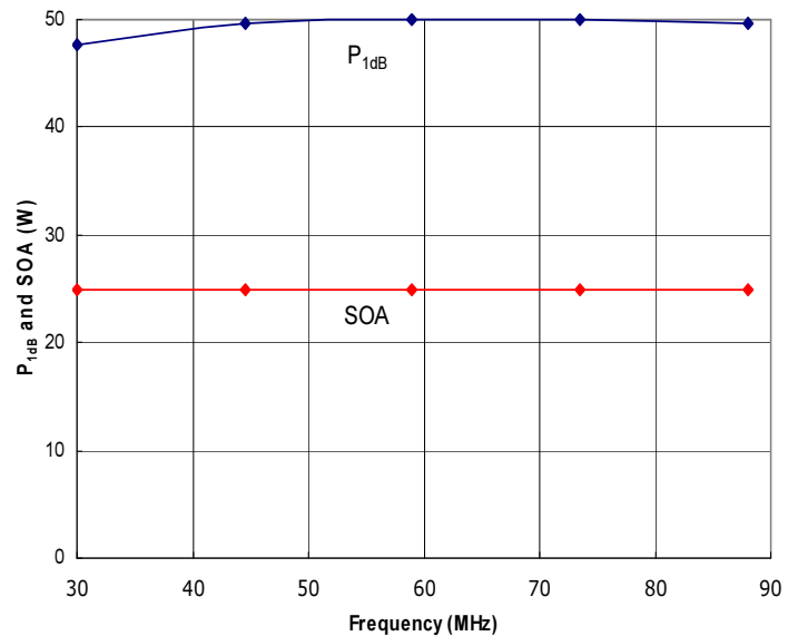
Figure 4: RFPS30-88-25 Typical P 1dB and Safe Operating Area (SOA). The amplifier is capable of delivering much more power than it is safe to generate. Do not exceed the SOA shown above.
