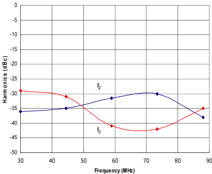
Figure 3: RFPS30-88-25 Typical f 2 and f 3 @ P out = 25W.
