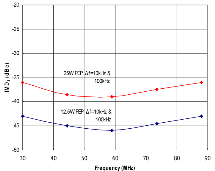
Figure 2: RFPS30-88-25 Typical IMD 3 , @ 25W and 12.5W PEP, Δf=10kHz and Δf=100kHz. Data is identical for both tone separations.
