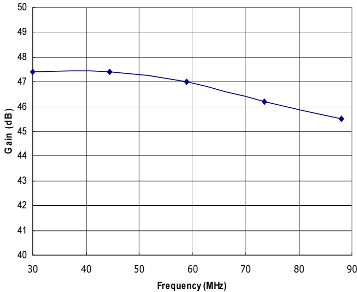
Figure 1: RFPS30-88-25 Typical Gain @ P out = 25W.
