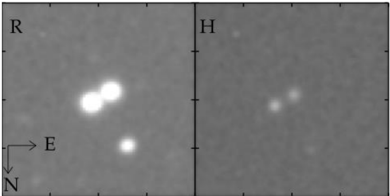
Figure 1. Example images of J 838 from the T11 telescope of the iTelescope network. Left: R filter. Right: H-alpha filter. The distance between divisions marked on the edge is 15'' .
