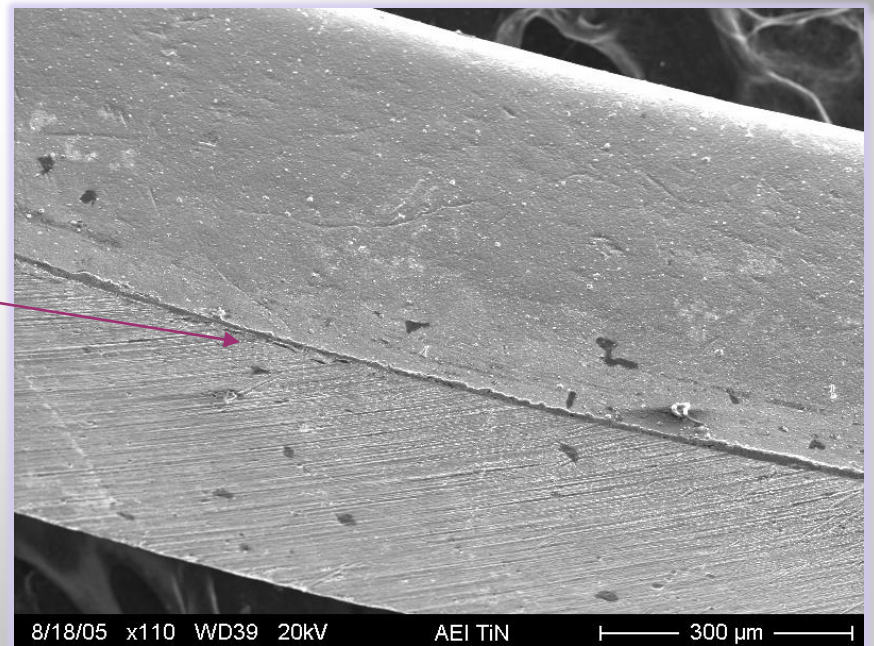
American Eagle Curette cutting edge after abrasion against Hu-Friedy Everedge Curette's cutting edge.
