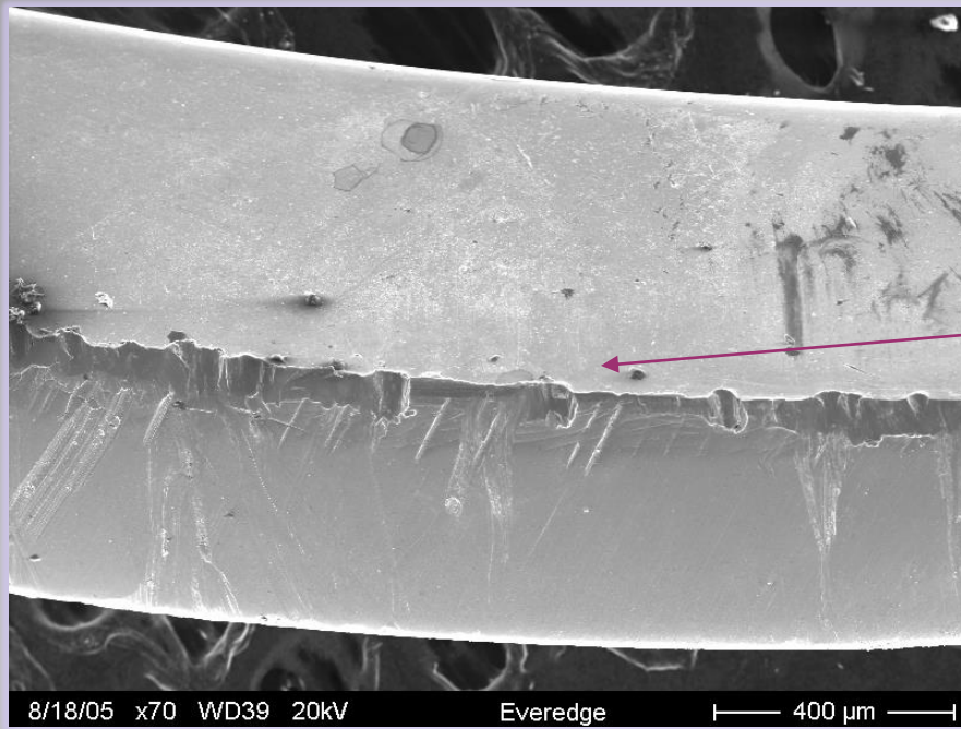
Hu-Friedy Everedge Curette cutting edge after abrasion against American Eagle's XP Technology surface- engineered cutting edge.
