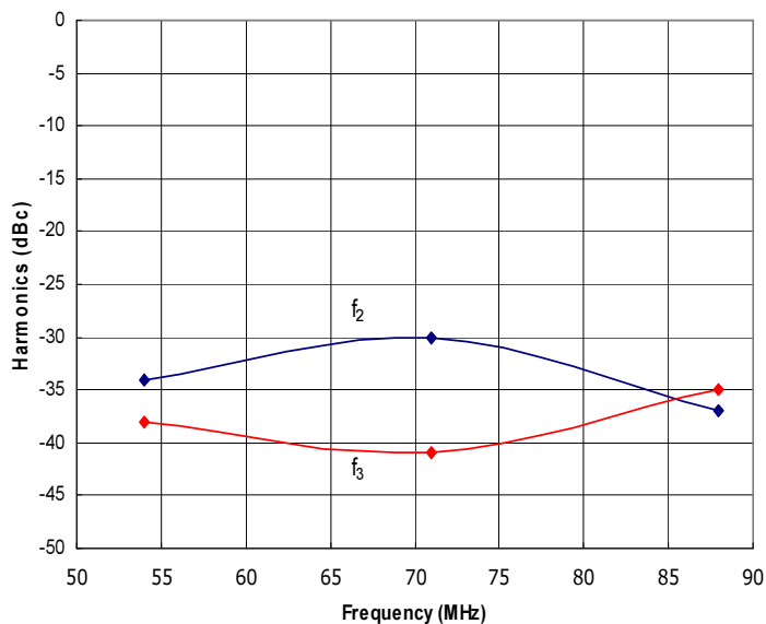
Figure 3: RFPS54-88-25 Typical f 2 and f 3 @ P out = 25W.
