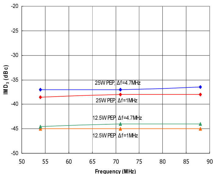
Figure 2: RFPS54-88-25 Typical IMD 3 , @ 25W and 12.5W PEP, Δf=1MHz and Δf=4.7MHz.
