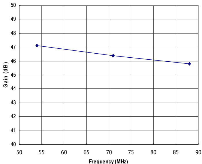
Figure 1: RFPS54-88-25 Typical Gain @ P out = 25W.
