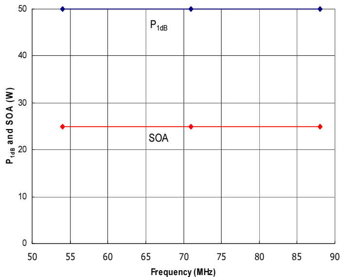
Figure 4: RFPS54-88-25 Typical P 1dB and Safe Operating Area (SOA). The amplifier is capable of delivering much more power than it is safe to generate. Do not exceed the SOA shown above.
