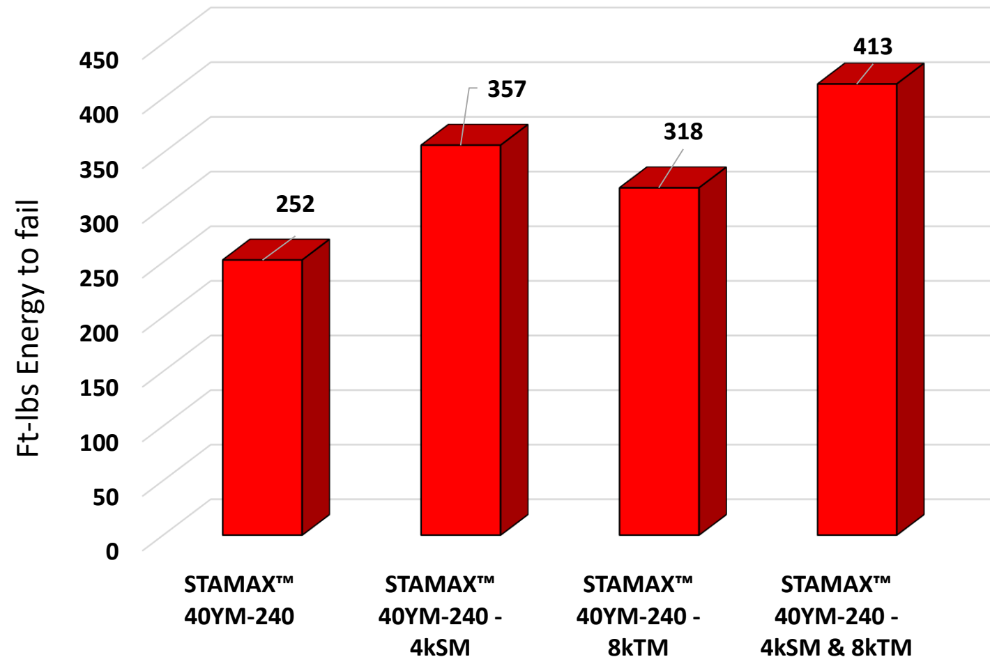
Compression Molded ICP 8"x18" Test Panels Impact Data - Pendulum Tester
