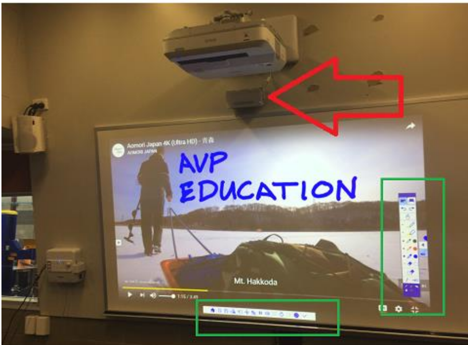
'NEW - 2018' Epson EB-695Wi (Pen and Finger touch – RED arrow shows the 'finger touch' unit installed);
