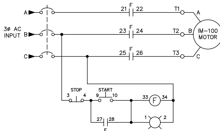
IM-100 Diagram
