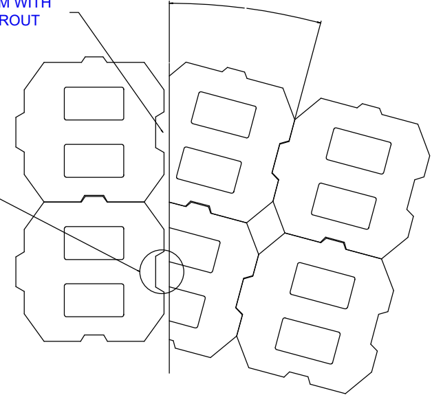
ANGLE MAT CONNECTION
