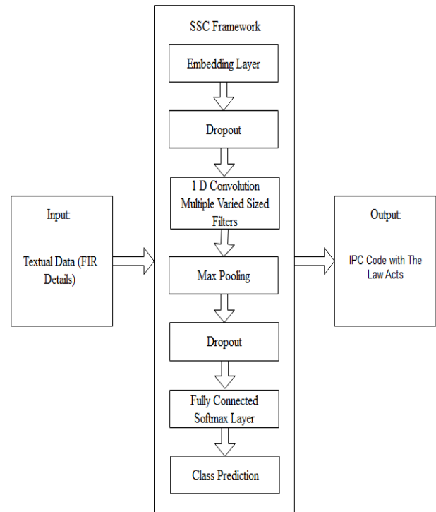
Fig. 1 System Architecture
