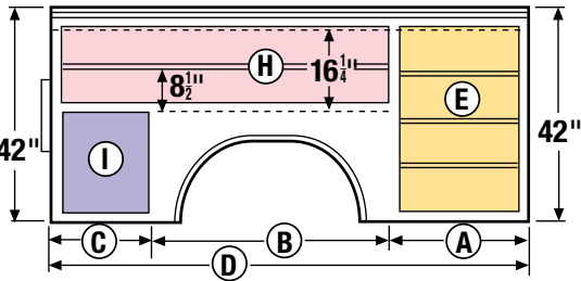
"B" Compartment Layout †
