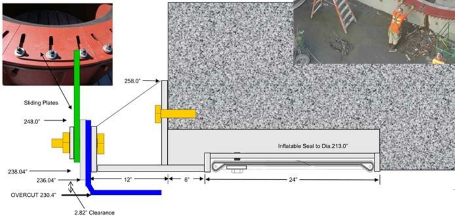
A 4 ply reinforced seal inflated with water forms a structural non-compressible bag (Oval)
