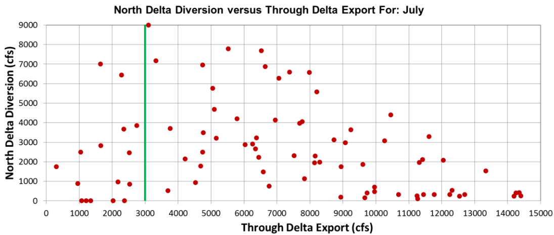
Figure 22. Alt 4-ELT North Delta Diversion Versus South Delta Diversion for July, August, and September
