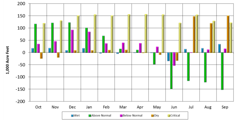
Figure 48. Oroville Reservoir Carryover Storage and Average Monthly Changes in Storage by Water Year Type
