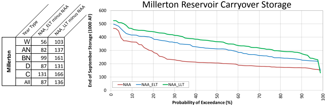
Figure 4. Millerton Reservoir Carryover Storage, NAA, NAA-ELT and NAA-LLT Scenarios
