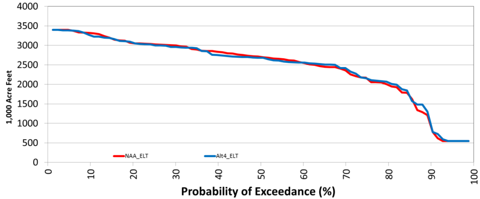
Figure 26. Shasta Reservoir Carryover Storage and Average Monthly Changes (Alt 4-ELT minus NAA-ELT) in Storage by Water Year Type
