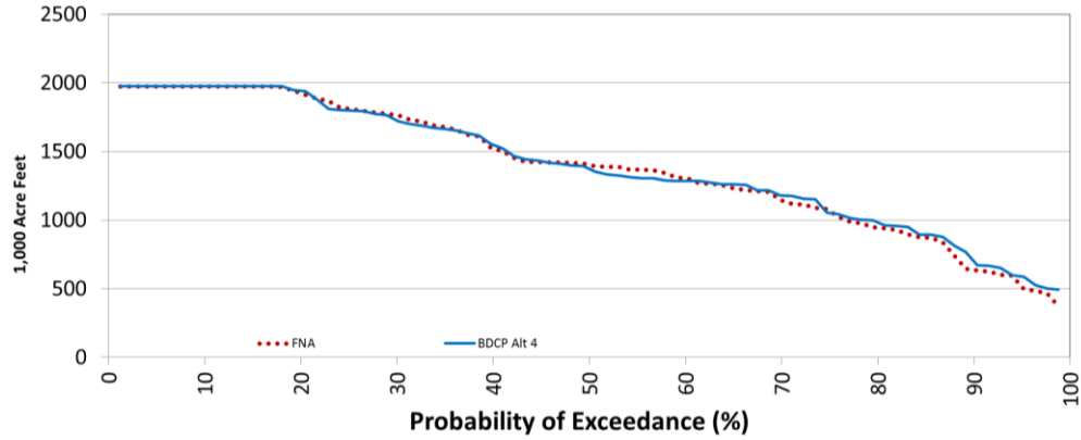
Figure 46. Trinity Reservoir Carryover Storage and Average Monthly Changes in Storage by Water Year Type
