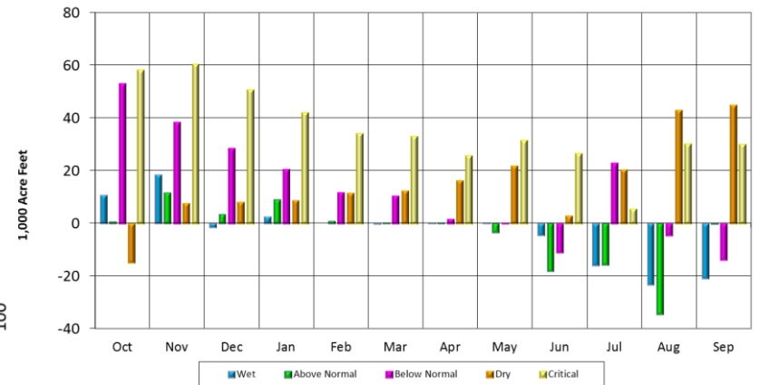
Figure 49. Folsom Reservoir Carryover Storage and Average Monthly Changes in Storage by Water Year Type
