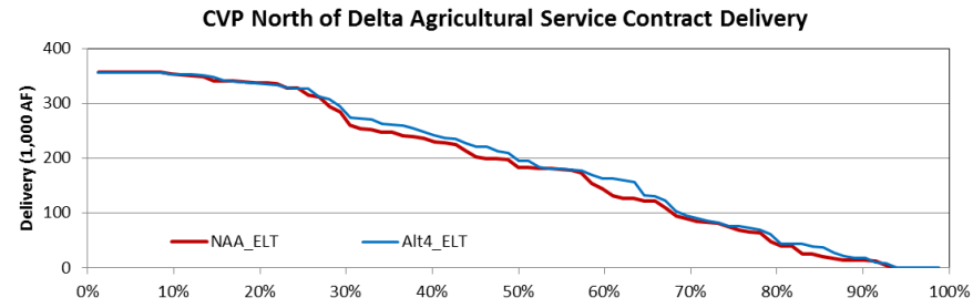
Figure 31. CVP Service Contract Deliveries (Alt 4-ELT and NAA-ELT)
