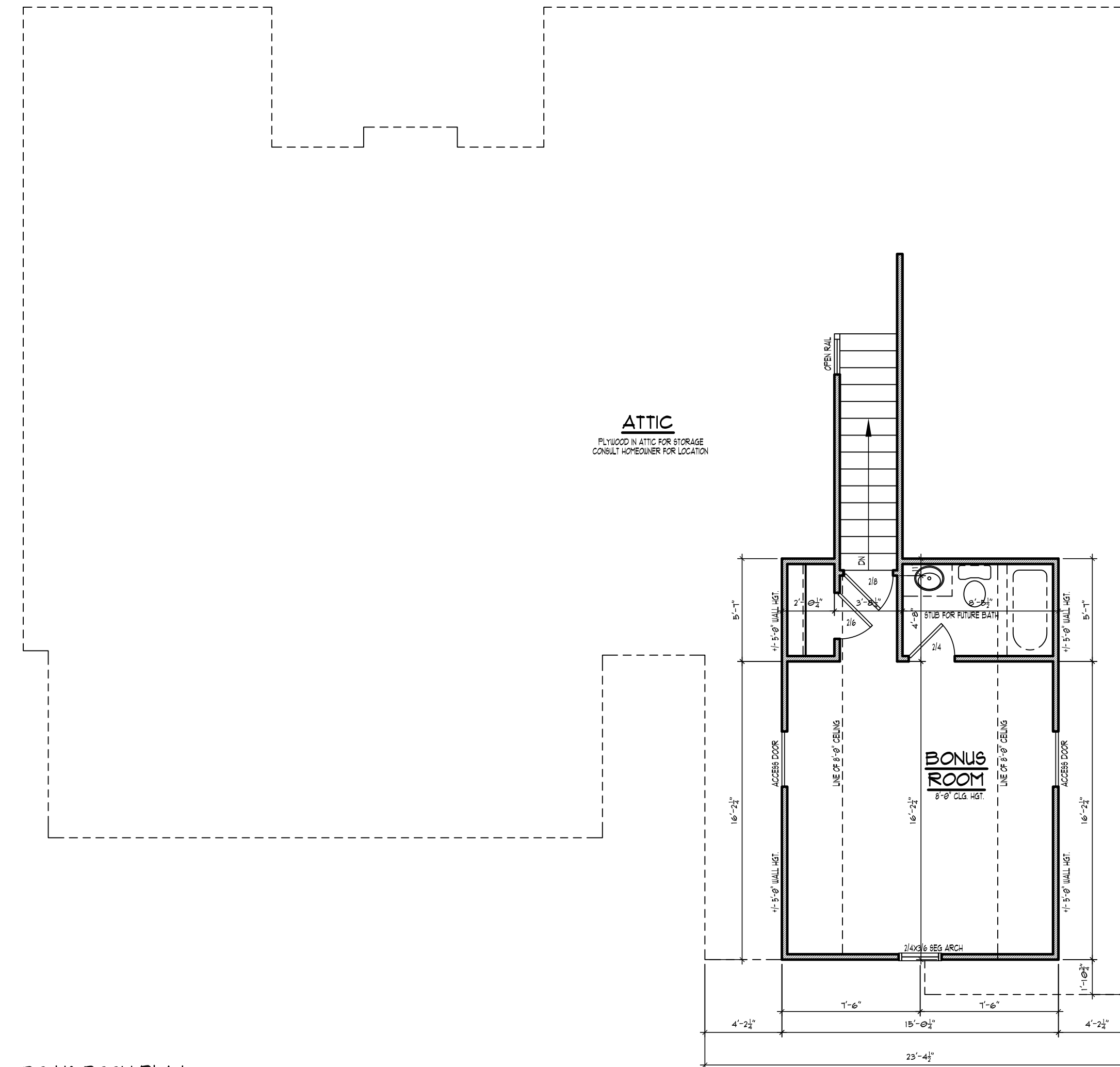
BONUS ROOM PLAN SCALE 1/4" = 1'-0"
