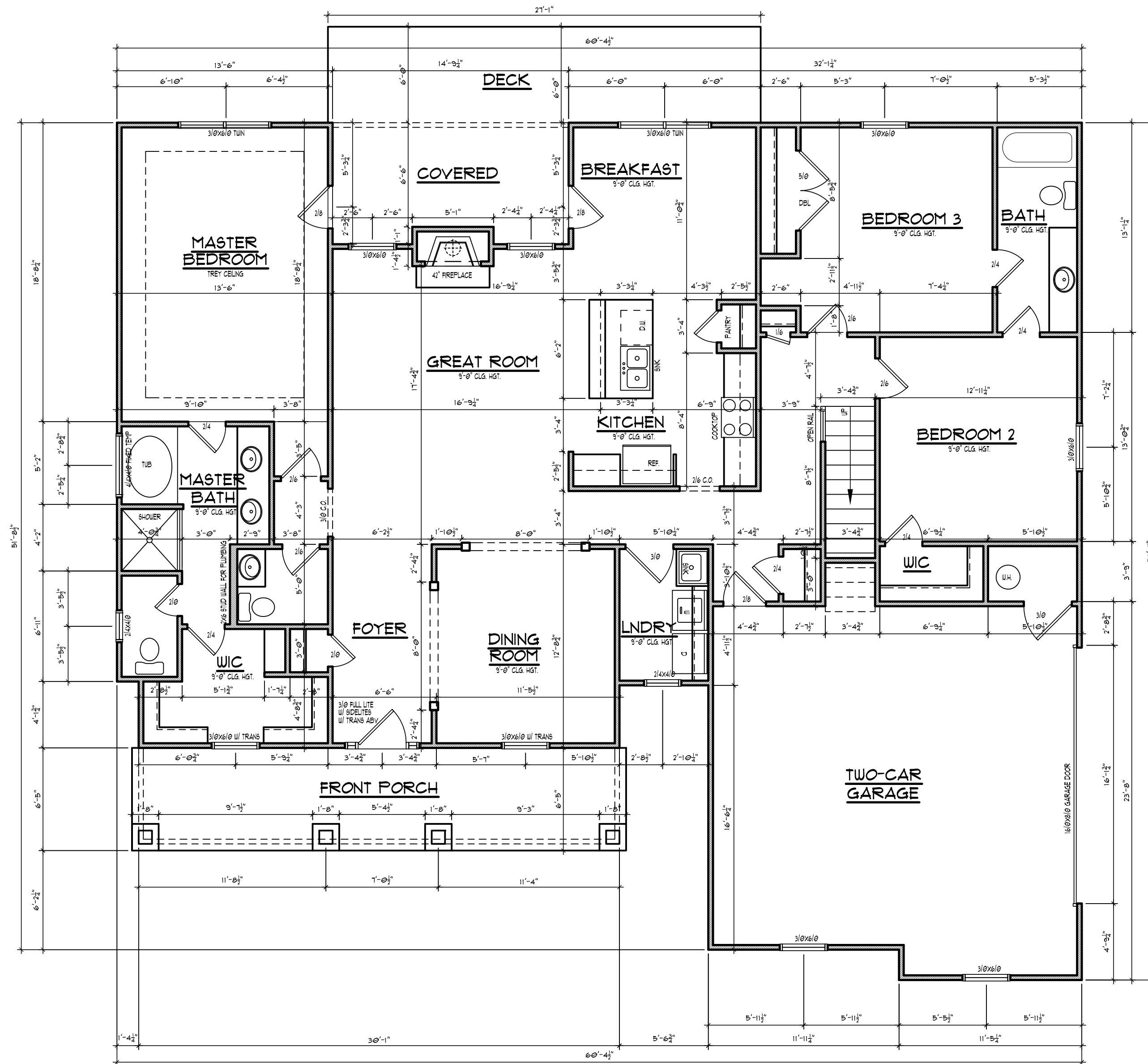
FIRST FLOOR SCALE 1/4" = 1'-0"
