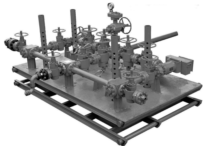
Cementing Manifold
