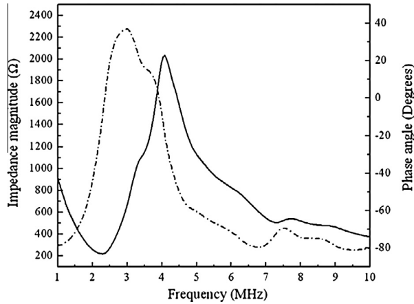
Fig. 13. Measured electrical impedance/phase for the PMN-PT single crystal array element. The solid and dotted lines represent the impedance and phase, respectively [90].
