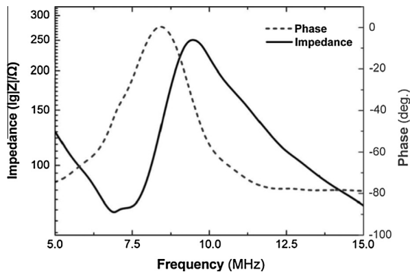
Fig. 18. Measured electrical impedance magnitude (solid line) and phase angle (dashed line) for a representative composite array element [96].
