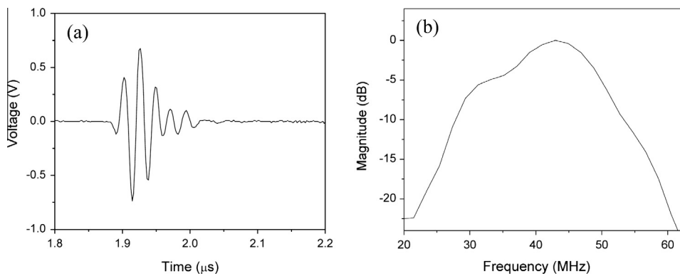
Fig. 6. (a) Measured pulse-echo waveform and (b) frequency spectrum for the 44-MHz PMN-PT needle transducer [81].
