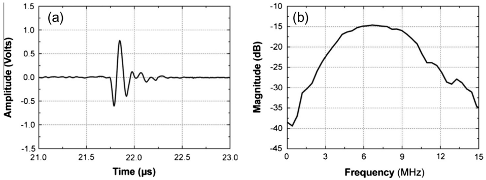
Fig. 19. Measured pulse-echo response for a representative composite array element [96].
