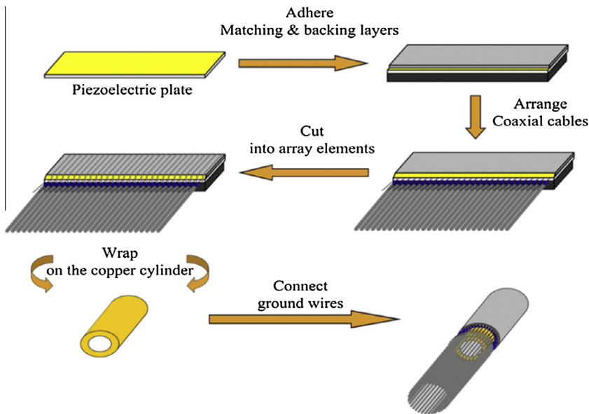
Fig. 16. Fabrication procedures of a PMN-PT/epoxy 1-3 composite radial array transducer [96].
