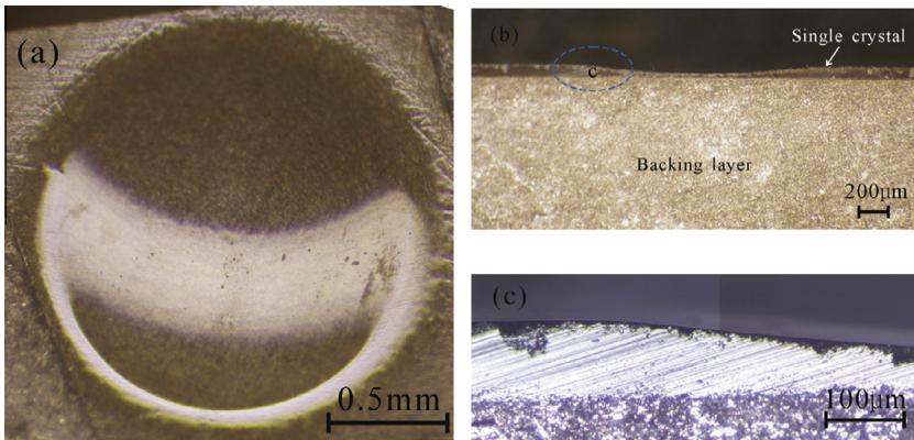
Fig. 4. Photographs of (a) top view, (b) cross section view and (c) a magnified cross section view of the dimpled PMN-PT single crystal with a backing layer [79].
