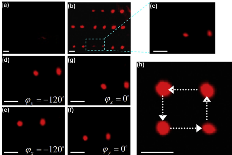
Fig. 30. The behavior of the MBs in the microfluidic device (a) prior to and (b) after application of ultrasonic wave. (c) The enlarged image of the MB cluster. (d, f) Transportation of MB cluster along the Y direction. (e, g) transportation of MB cluster along the X direction. (h) the composite image shows the trajectory of the MB cluster. The scale bar is 20 \mu\text{m} [111].
