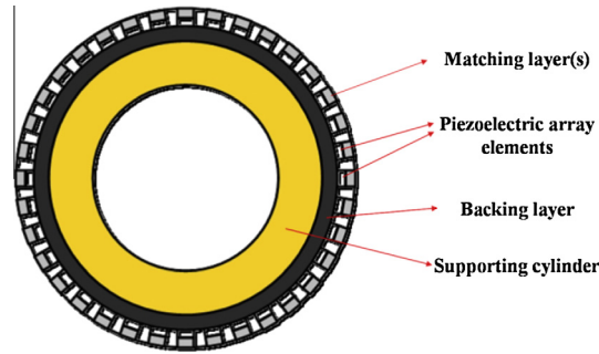
Fig. 15. Schematic cross section view of a radial array transducer [96].
