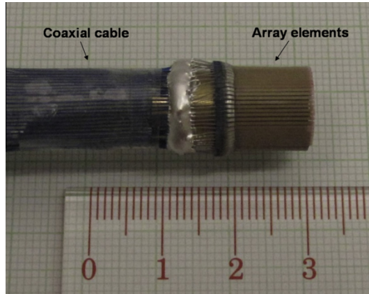
Fig. 17. Photograph of a PMN-PT/epoxy 1-3 composite radial array transducer [96].
