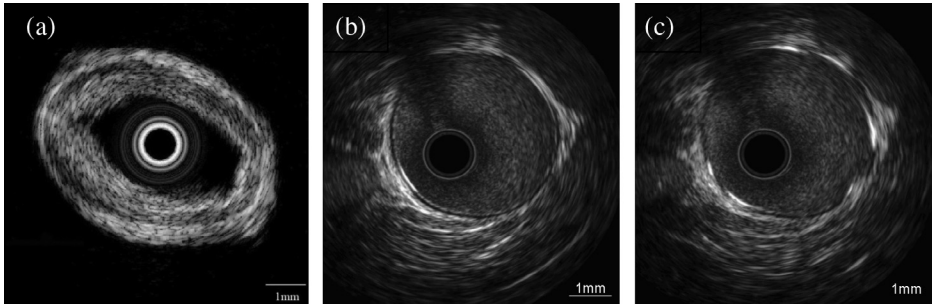
Fig. 21. (a) In vitro imaging of human coronary artery acquired by a 32-MHz PMN–PT single crystal catheter. (b) Intravascular image of a porcine vessel taken with a 60-MHz 1-3 composite based transducer. (c) Intravascular image of a porcine vessel with stent taken with a 60-MHz 1-3 composite based transducer [98].
