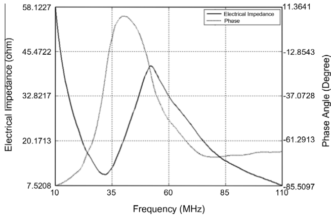
Fig. 9. Measured electrical impedance/phase for the PMN-PT single crystal/epoxy 1-3 composite transducer [88].
