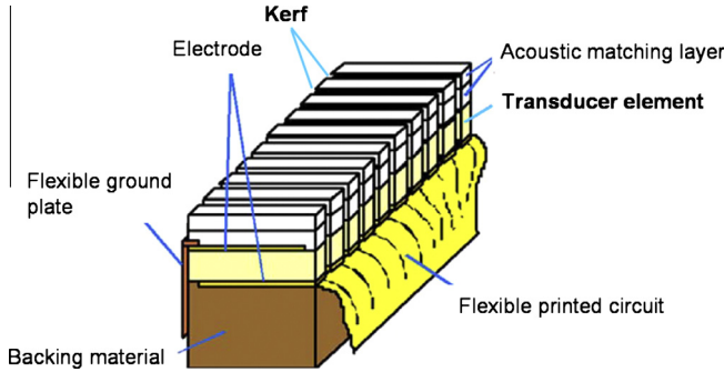
Fig. 11. Schematic diagram of a linear array transducer [90].
