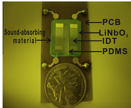
Fig. 29. Photograph of the microfluidic device. LN crystal is used as a substrate to generate ultrasonic wave because of its high coupling coefficient [110].
