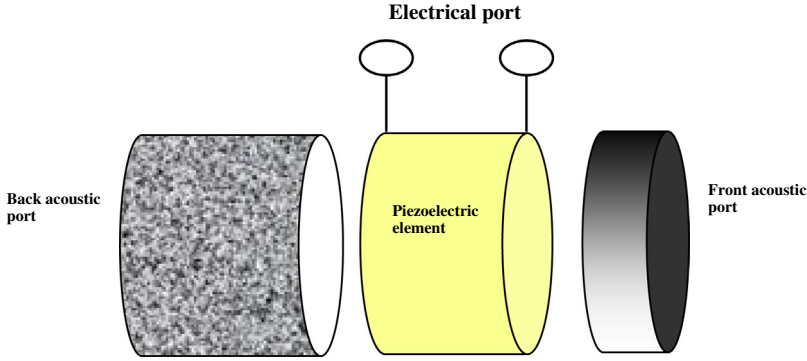
Fig. 1. A three-port network of the transducer [1].
