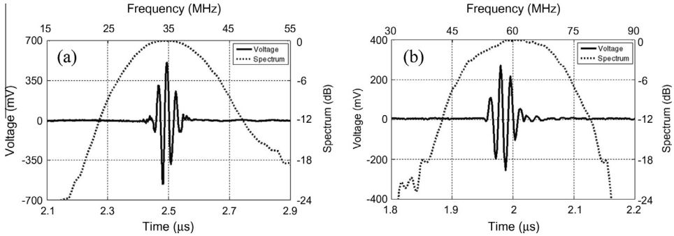
Fig. 7. Measured pulse-echo waveform and spectrum for the (a) 35 MHz and (b) 60 MHz PIN-PMN-PT piston transducer [74].
