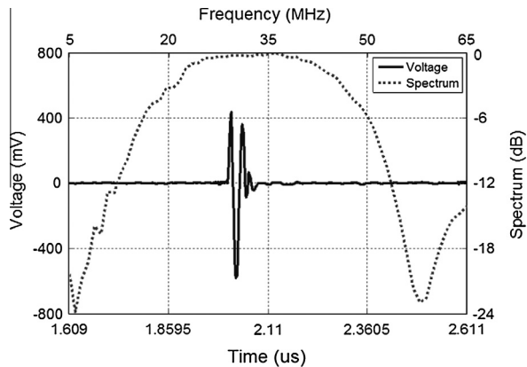
Fig. 10. Measured pulse-echo impulse response and frequency spectrum of the PMN-PT single crystal/epoxy 1-3 composite transducer [88].
