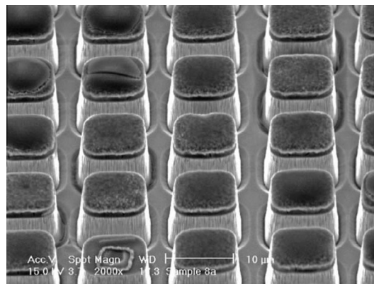
Fig. 8. SEM micrograph of the etched PMN-PT single crystal [88].
