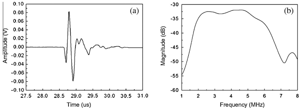
Fig. 14. (a) Measured pulse-echo impulse response and (b) frequency spectrum of the PMN-PT single crystal array element [90].
