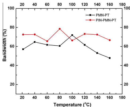
Fig. 12. Comparison of -6\text{ dB} bandwidth of PMN–PT and PIN–PMN–PT single crystal linear array transducers [91].
