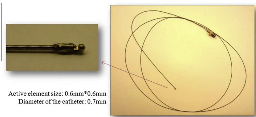
Fig. 5. Side-view of miniature plane transducer designed for intravascular imaging application [80].
