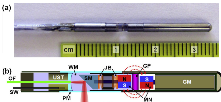
Fig. 26. (a) Photograph of the integrated mini-probe's rigid distal end. (b) Schematic of the mini-probe. GM, geared micromotor; GP, glass partition; JB, jewel bearings; MN, magnets; OF, optical fiber; PM, plastic membrane (imaging window); SM, scanning mirror; SW, signal wire; UST, ultrasonic transducer; WM, water medium [106].
