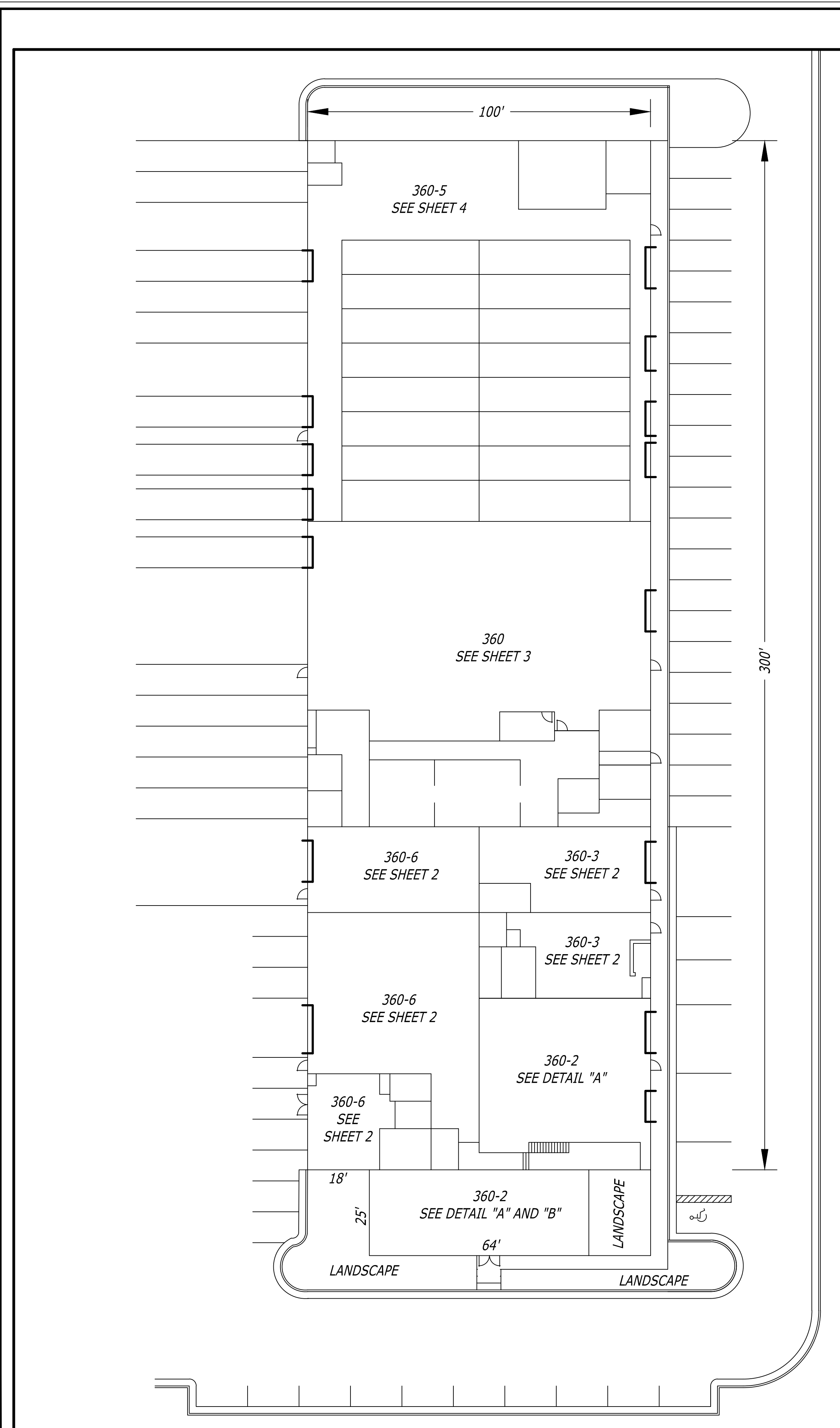
SCALE 1"=20'
