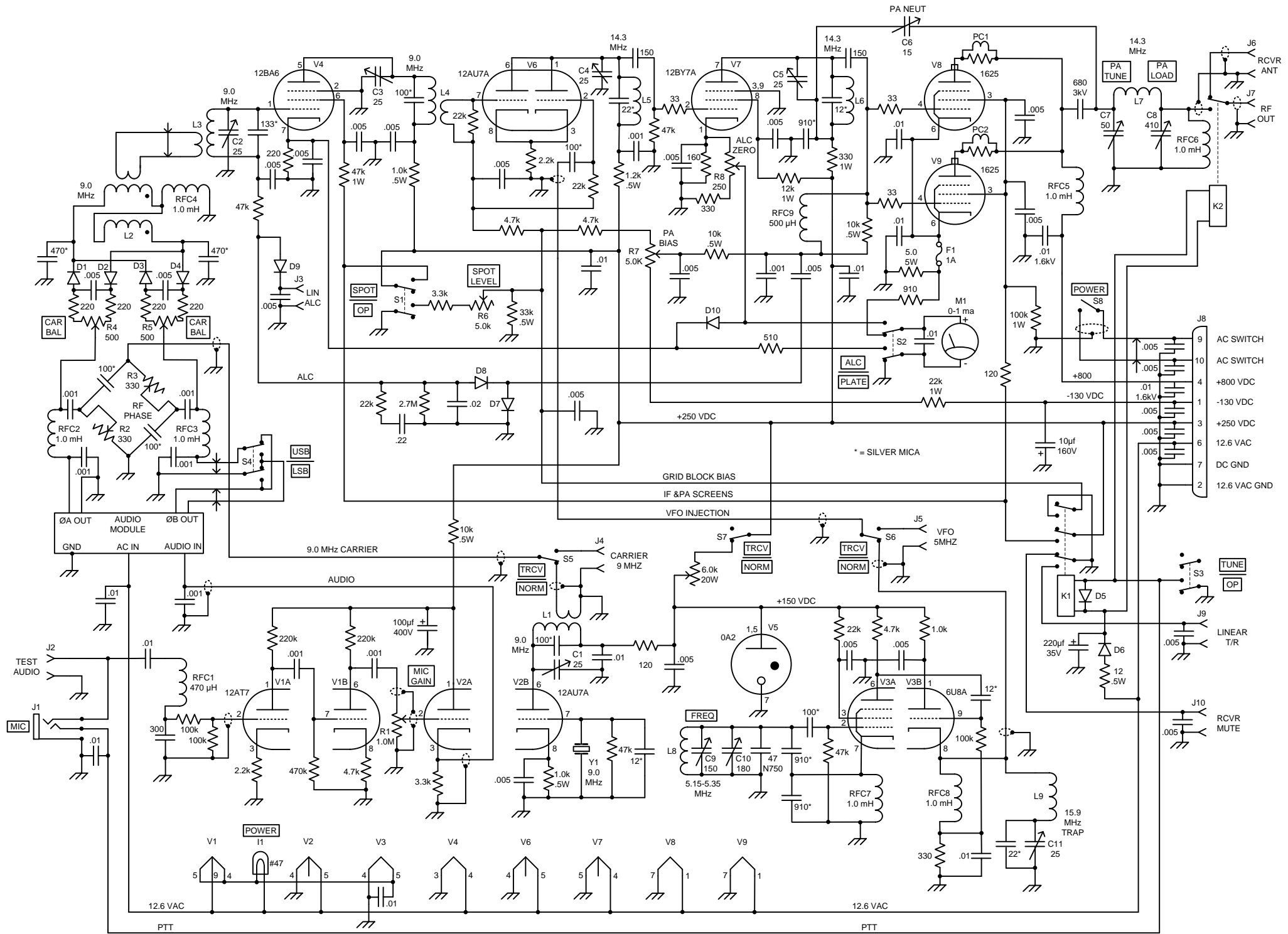
TRANSMITTER SCHEMATIC
