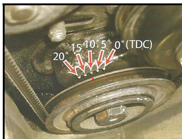
Figure 18 – Timing Marks
