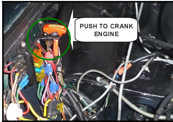
Figure 12 – Remote Cranking
