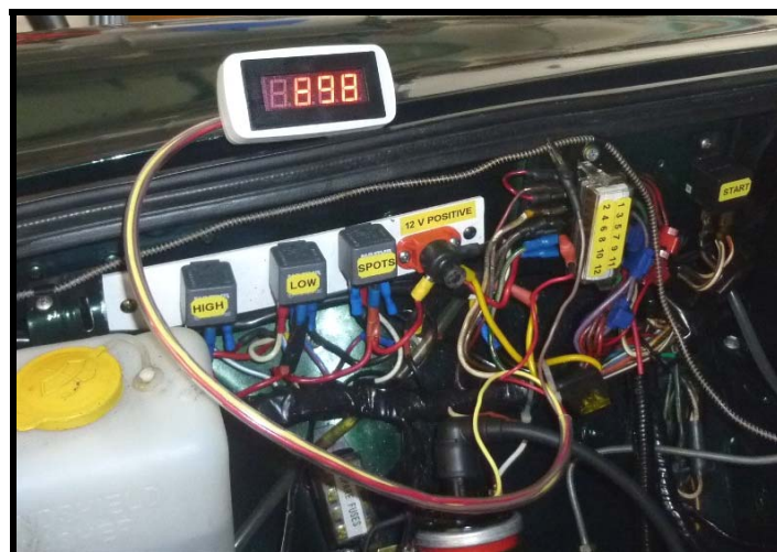
Figure 15 – Tachometer
