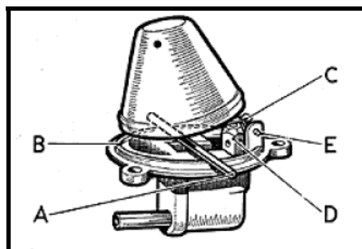
Figure 38 – Fuel Float (from Bentley manual)
