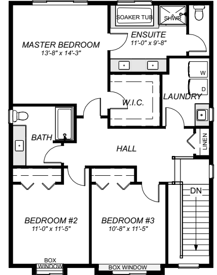
UPPER FLOOR PLAN 1141 sq ft
