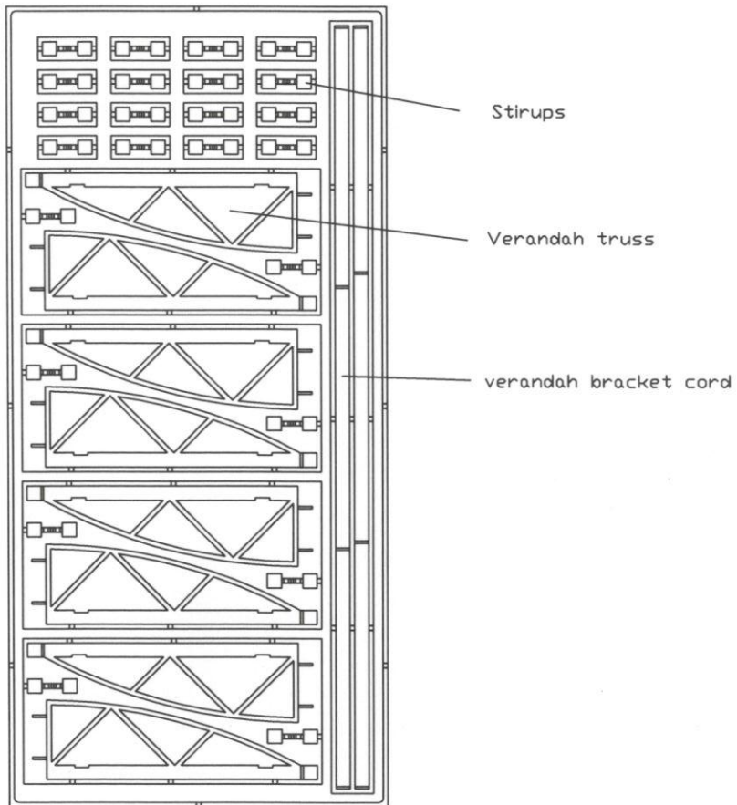
400 mm Verandah Frame
