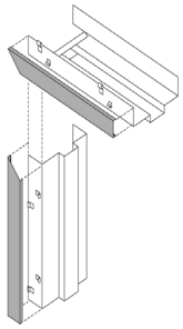
CORNER DETAIL
