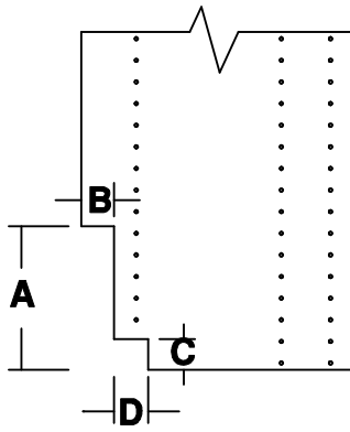
BASE NOTCH "B"
