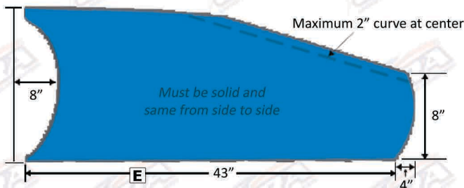
Spoiler Braces
