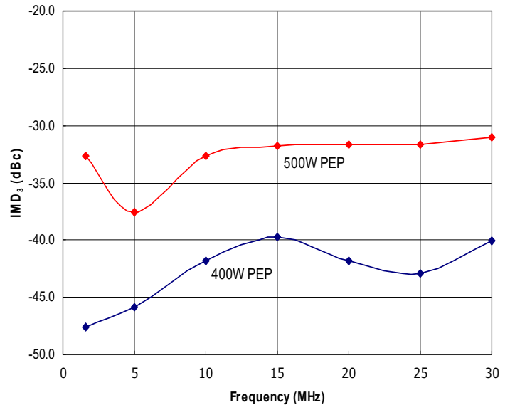
Figure 2: RFP1.6-30-500XR Typical IMD 3 @ Δf=10kHz, 500W PEP and 400W PEP.
