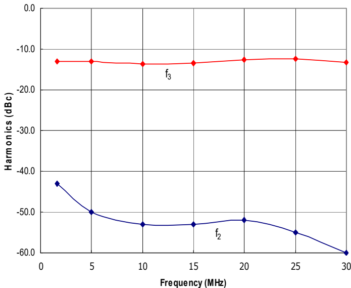
Figure 3: RFP1.6-30-500XR Typical f 2 and f 3 @ P out = 500W.
