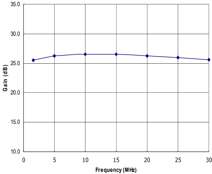
Figure 1: RFP1.6-30-500XR Typical Gain @ P out = 500W.
