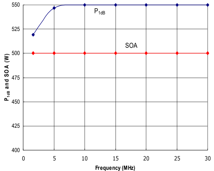
Figure 4: RFP1.6-30-500XR Typical P 1dB and Safe Operating Area (SOA). Do not exceed the SOA shown above without first contacting RFMPT to discuss your application.
