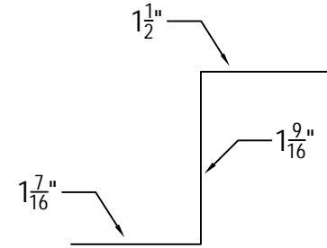
STANDING SEAM SAW CUT REGLET _____ LINEAR FEET (120" PCS)
