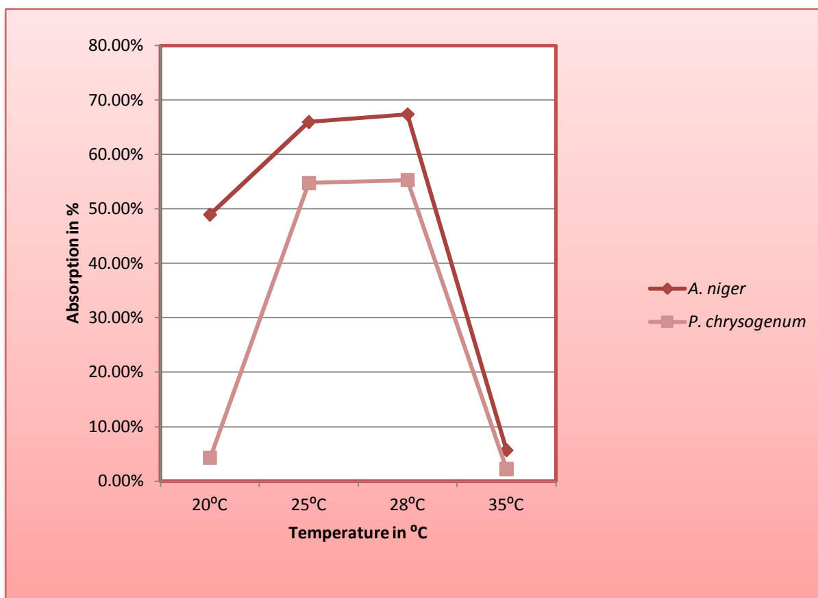
Fig 3: Effects of different temperature (in °C.) on absorption of iron by A.niger and P.
