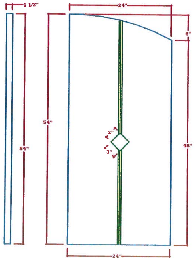
A SHUTTER 8
