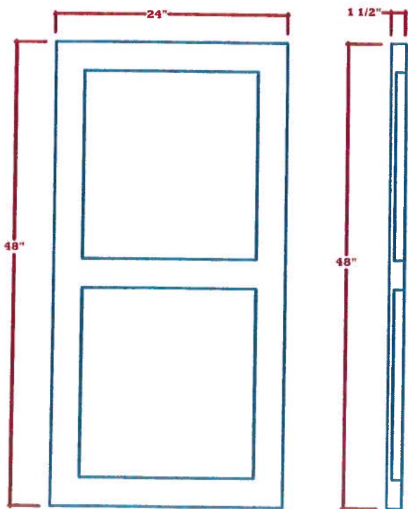
A SHUTTER 16
