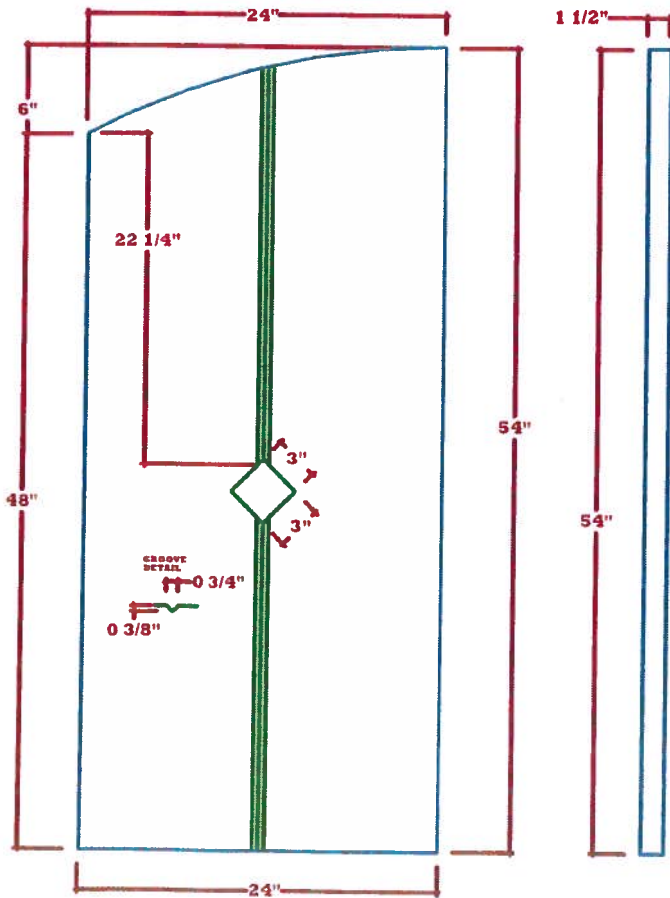
A SHUTTER 7
