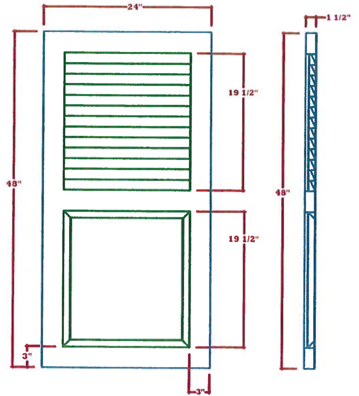
A SHUTTER 15
