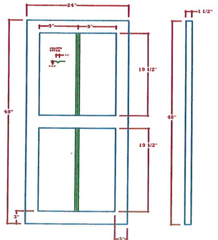
A SHUTTER 17
