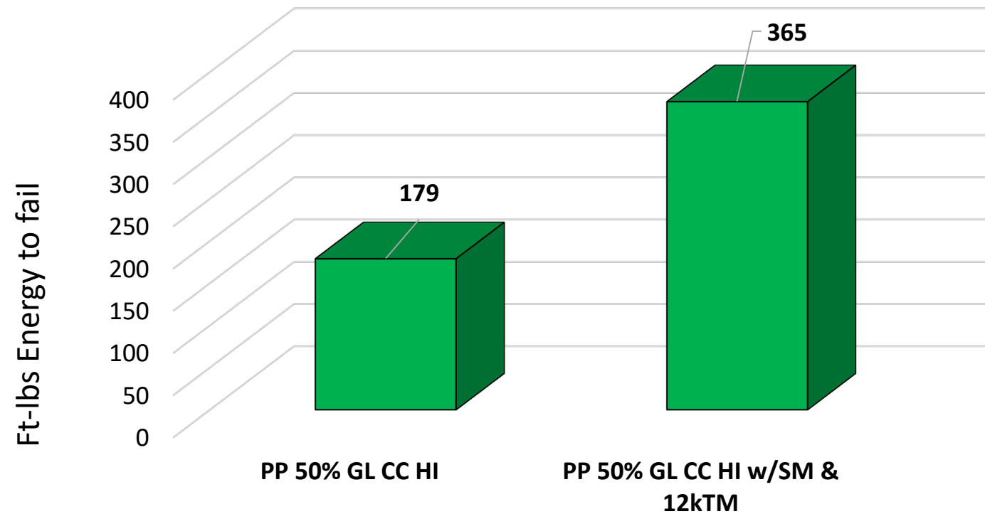
Injection Molded ICP 5" Test Panels Impact Data - Pendulum Tester
