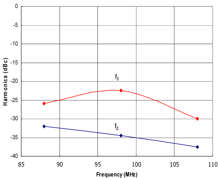
Figure 3: RFPS88-108-50 Typical f 2 and f 3 @ P out = 50W.
