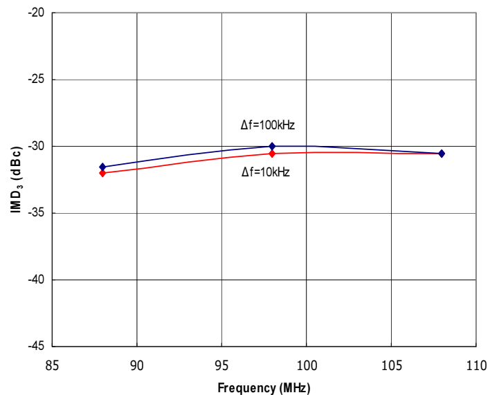
Figure 2: RFPS88-108-50 Typical IMD 3 @ 50W PEP, Δf=10kHz and Δf=100kHz. Data is provided for reference only; this is not intended to be a highly linear amplifier. For improved linearity, see our RFPS88-108-25 Class A amplifier.
