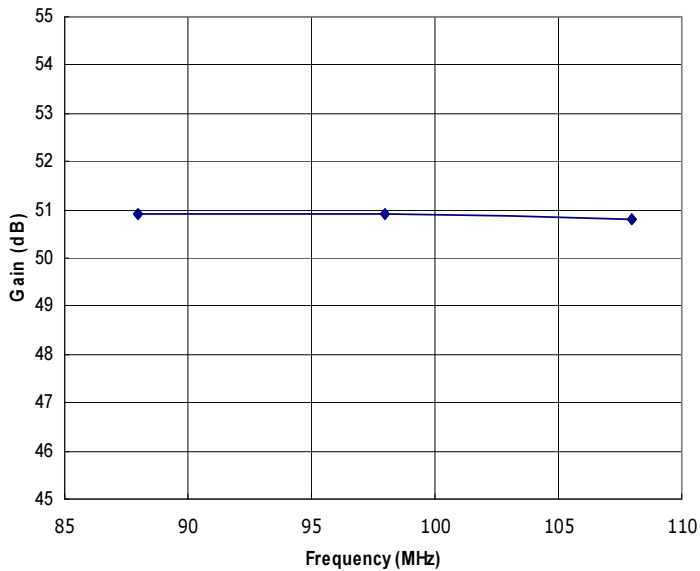
Figure 1: RFPS88-108-50 Typical Gain @ P out = 50W.
