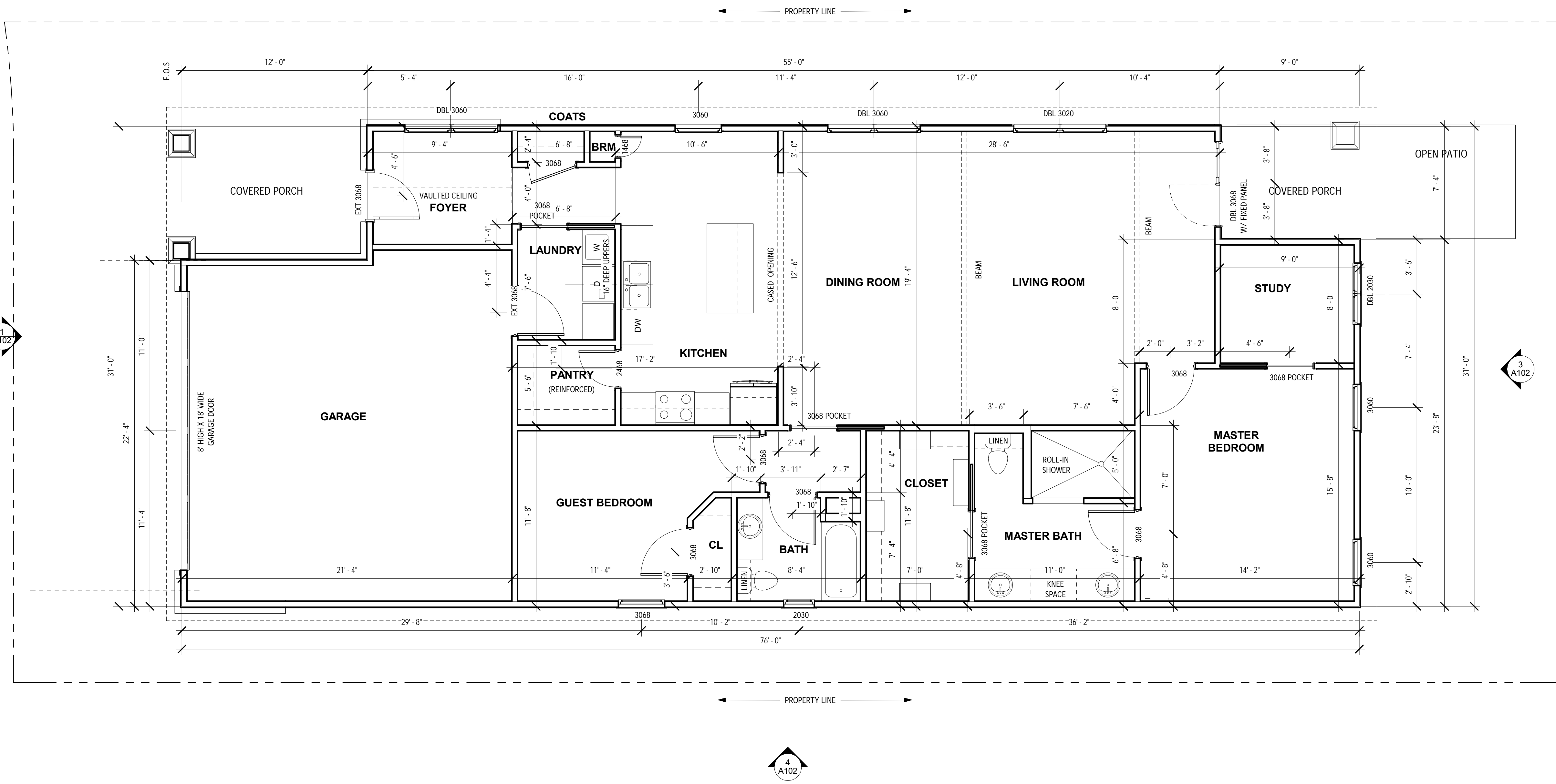
1 FLOOR PLAN 1/4" = 1'-0"
