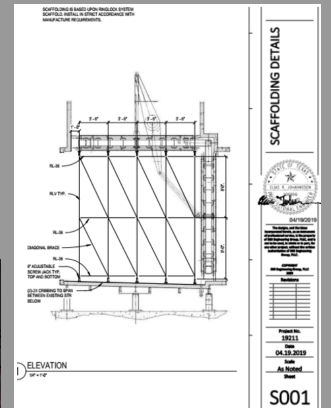
PE Stamped Shoring Solution
