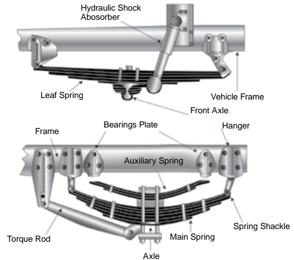
Figure 2-2: Key Suspension Parts
