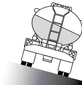
Figure 8-2: Shifting cargo
