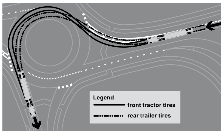
Figure 2-16d: Lane separation, wide gore, left turn
