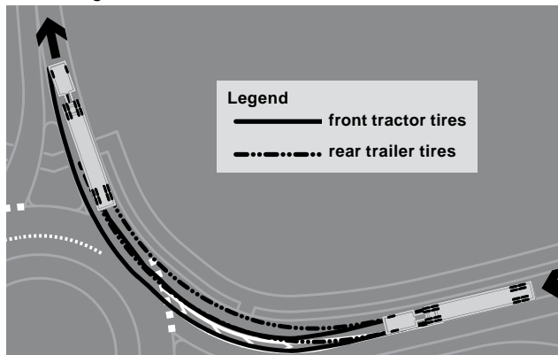
Figure 2-16f: Lane separations, wide gore, through movement.
