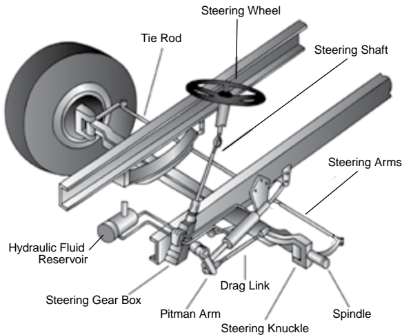
Figure 2-1: Steering System
