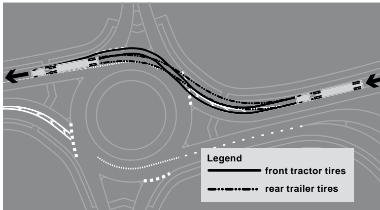
Figure 2-16e: Lane separation, wide gore, right turn
