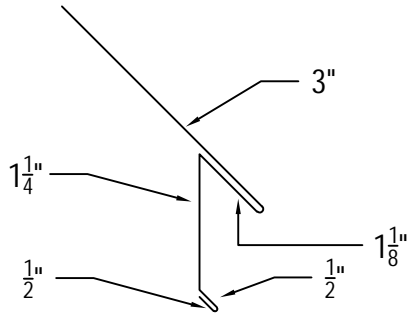
STANDING SEAM DRIP EDGE _____ LINEAR FEET (120" PCS)
