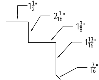
STANDING SEAM RAKE CLEAT _____ LINEAR FEET (120" PCS)
