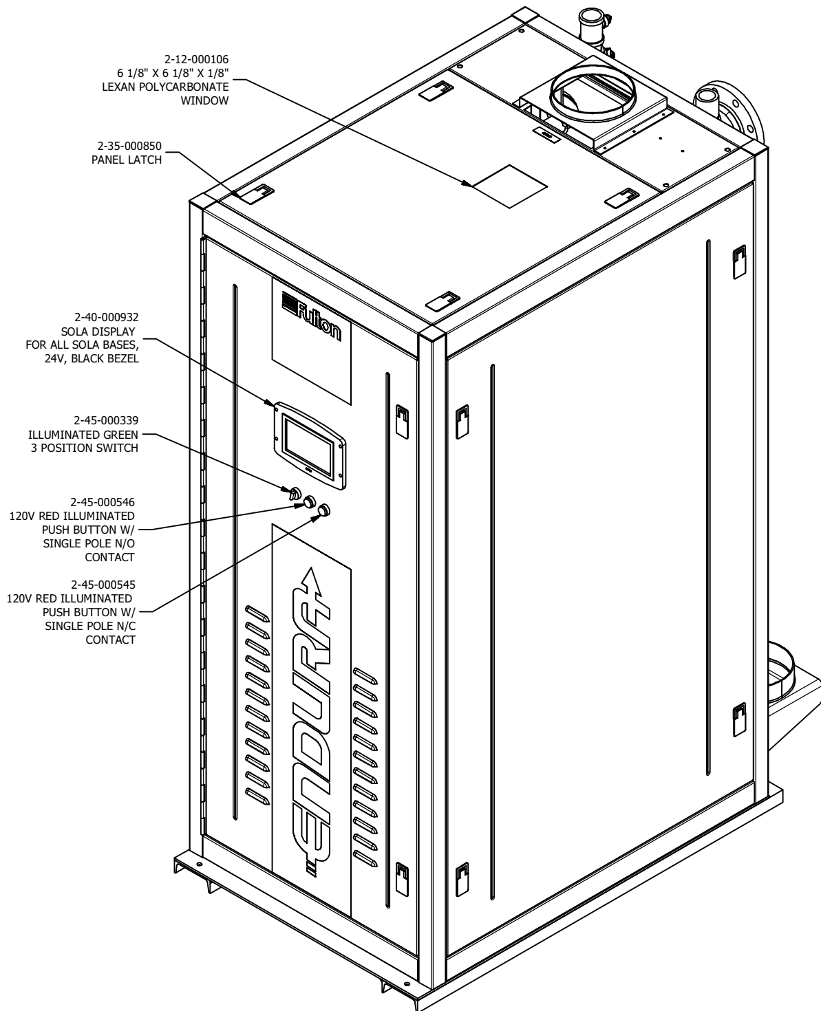
ENDURA 2000K ISOMETRIC
