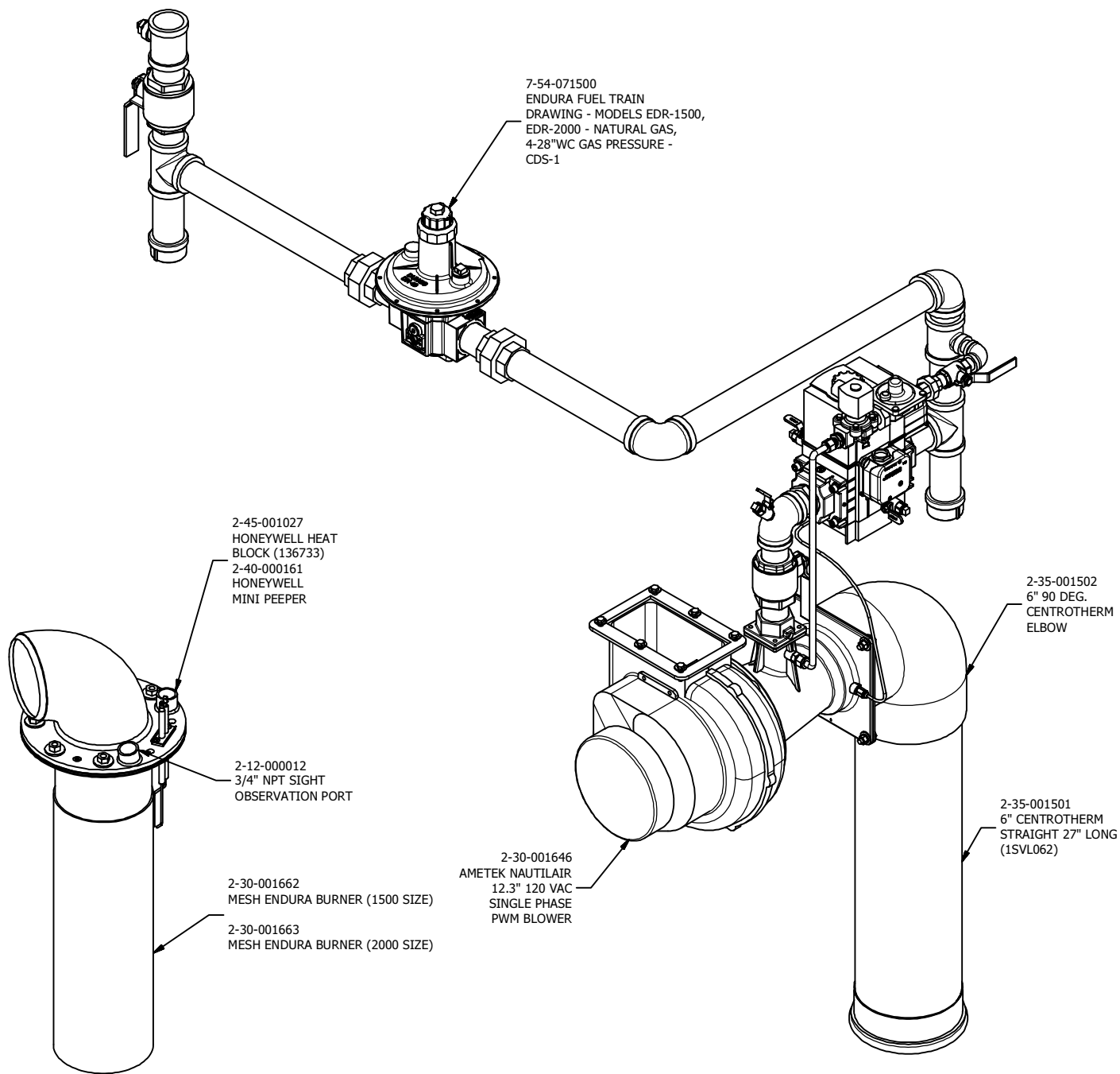
IGNITION DETAIL VIEW
