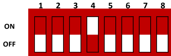
Figure 14: S1/S4 Rsl setting for 10000Ω
