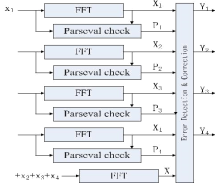
Fig.2: Parity-SOS (first technique) fault-tolerant parallel FFTs.
