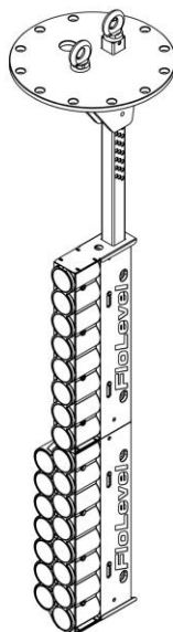
Single Standard Resolution and High Resolution Array Control range 0-1300mm (0-50")
