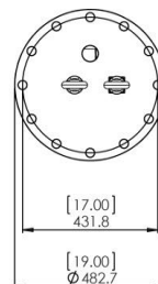
Single Array High Resolution Control range 0-650mm (0-25")
