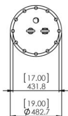
Single Standard Resolution and High Resolution Array Control range 0-1300mm (0-50")
