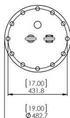
Single Array Standard Resolution Control range 0-650mm (0-25")
