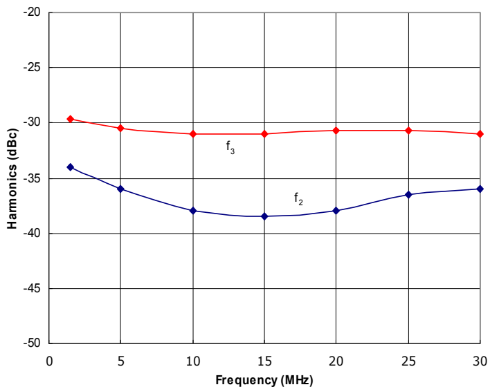
Figure 3: RFM1.5-30-25-HSD Typical f 2 and f 3 @ P out = 25W.
