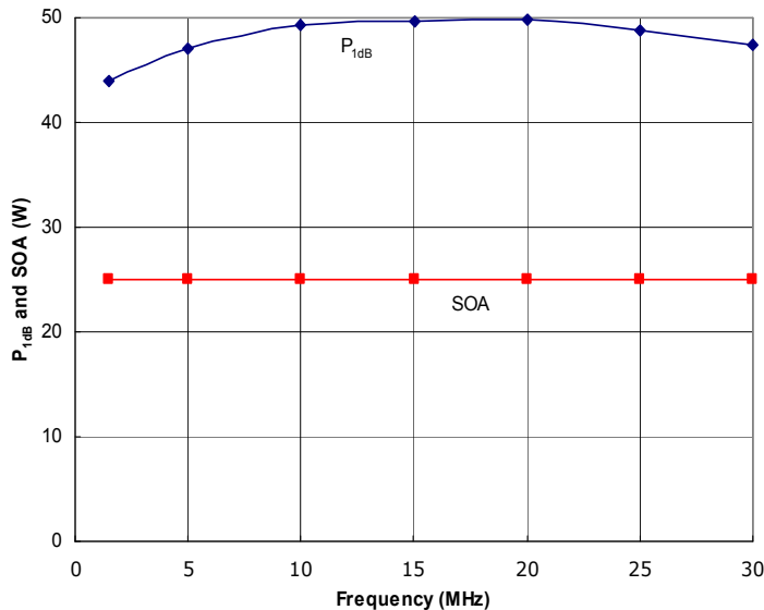
Figure 4: RFM1.5-30-25-HSD Typical P 1dB and Safe Operating Area (SOA). The amplifier is capable of delivering much more power than it is safe to generate. Do not exceed the SOA shown above without first contacting RFMPT to discuss your application.
