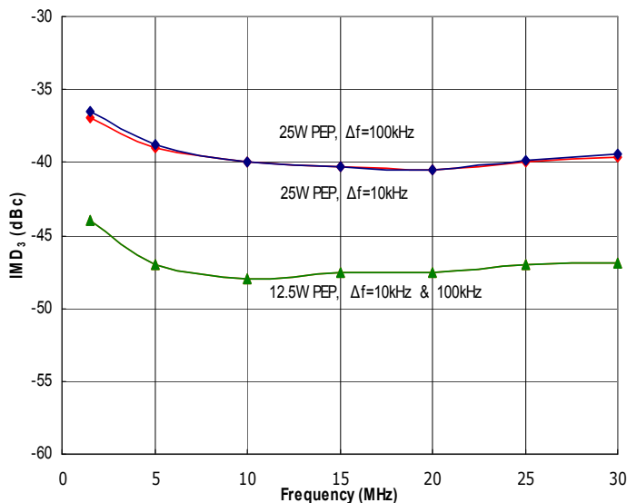
Figure 2: RFM1.5-30-25-HSD Typical IMD 3 @ 25W and 12.5W PEP, Δf=10kHz and Δf=100kHz.
