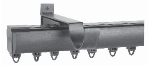
Double System with Back Traverse and Stationary Pole in Front
