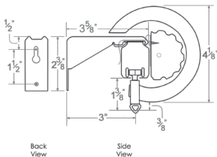
EZ50 3" EasyPull™ Single Bracket
