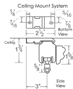
EZ52 EasyPull™ Ceiling Bracket
