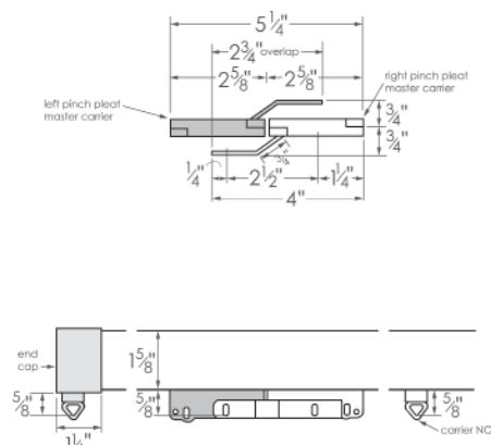
EZ55 Heavy-Duty Glide
