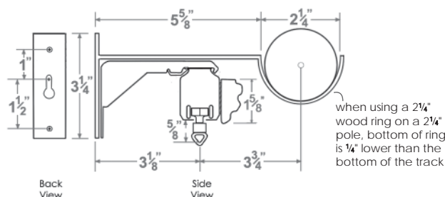
PO214OVBKS EasyPull™ Over Bracket
