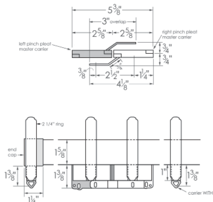
EZ54 Heavy-Duty Glide and C-Ring
