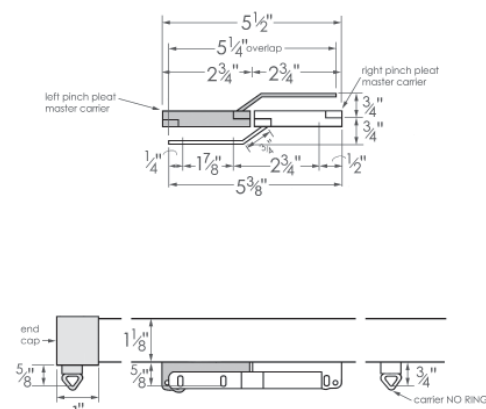
EZ59 Light-Duty Glide
