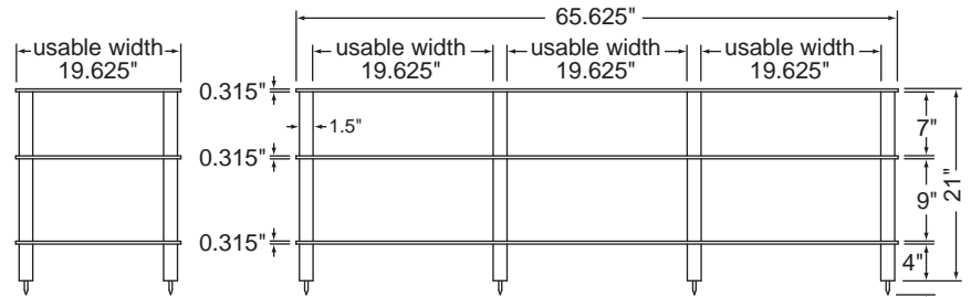
SIDE VIEW
