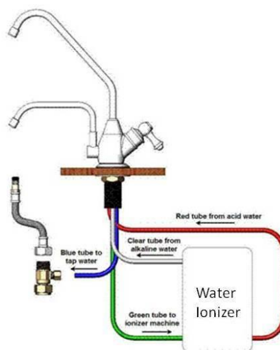
Dual Headed Under-sink Kit For Melody II, Athena H2, or Vesta H2
