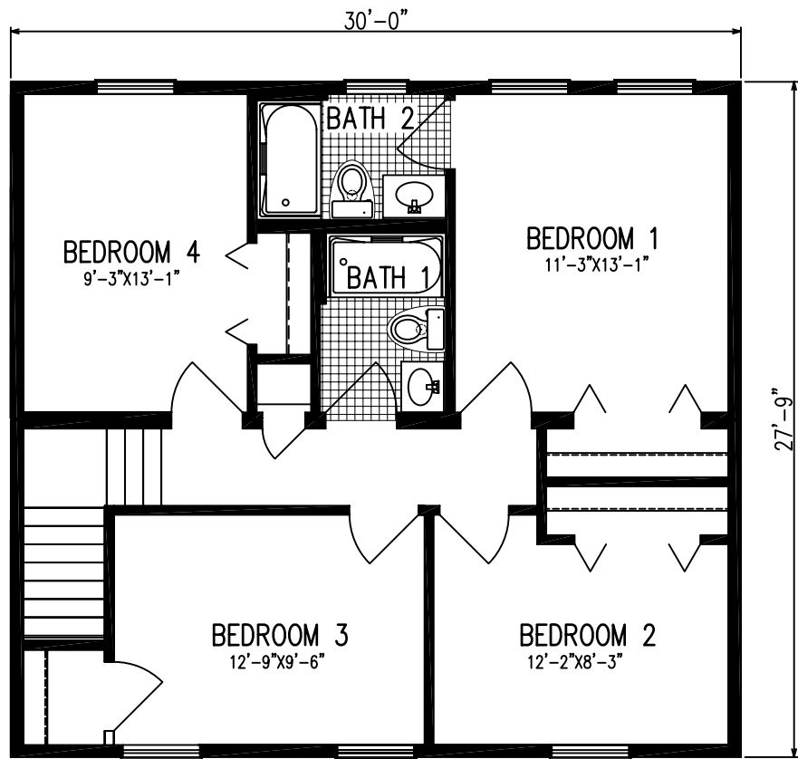
2ND FLOOR- 840 SQ FT
