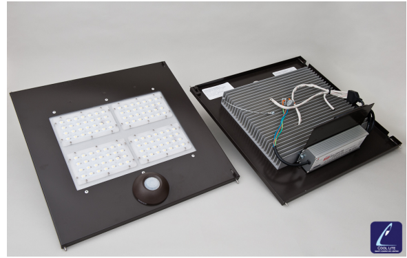
Gardco Form 10 Shoebox Retrofit Kit
