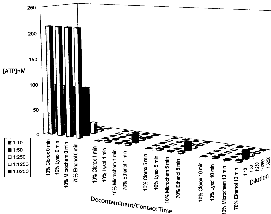
Fig. B-7. B. anthracis spore assay after suspension decontamination by the ATP-Glow method. The ATP measurement of B. anthracis spore suspensions were decontaminated with 10% Lysol™, 10% Clorox™, 10% Micro-Chem Plus™, or 70% ethanol, respectively.
