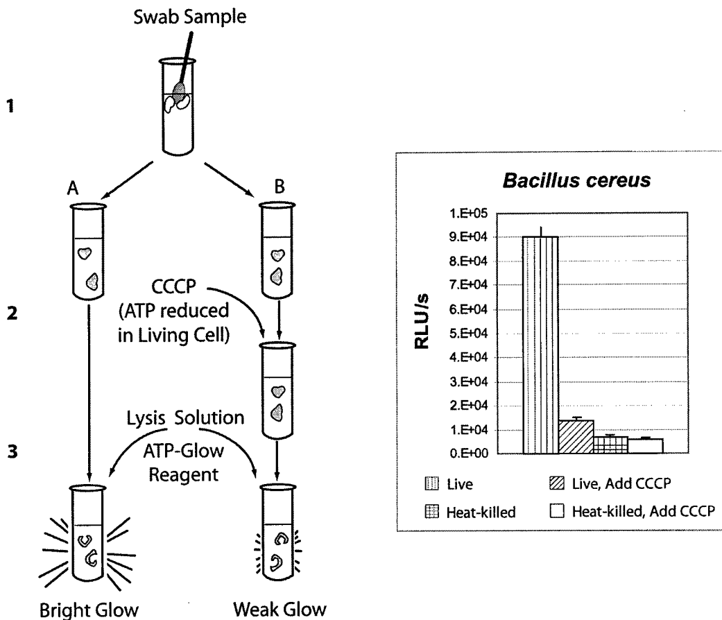
Fig. B-1. How does it work? The diagram shows the proposed ATP-Glow principle for the rapid & sensitive detection of viable bacterial spores and cells, and assessing the efficacy of decontamination. The assay procedure includes: 1. Add the swab sample (microorganisms) into probe solution; and distribute the solution into two tubes or wells (A & B); 2. Add CCCP solution to well B. 3. Add lysis solution and ATP-Glow solution into both A & B, and measure luminescence. The signal corresponds to the total ATP in the sample, and the decrease in luminescence in tube B is due to the effect of protonophores (CCCP) on live organisms. The Phase I Bacillus cereus data shows a significant CCCP effect on live cells, while negligible effect on dead cells (negative control). The decrease in luminescence is corresponds to the number of live cells. (see Sec. B.3.2.2 for details)
