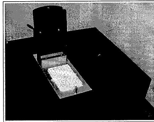
Fig. B-9 (a) The photo shows the MSI-ATP-Glow readout optoelectronics and mechanical components. (b) The exterior view of the prototype. The system will be further miniaturized in Phase II.
