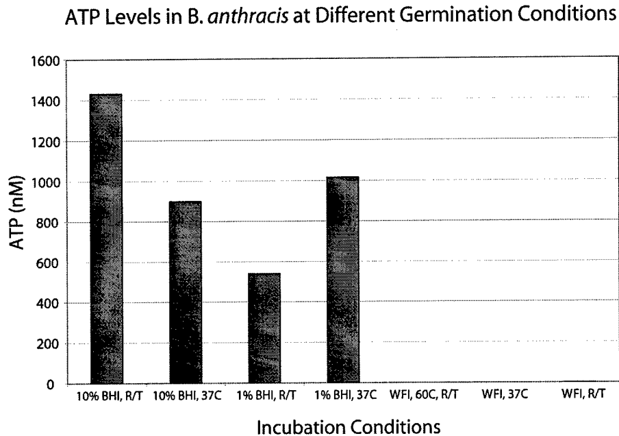
Figure B-5. The data show the concentration of ATP present in Bacillus anthracis spores under various incubation conditions.
