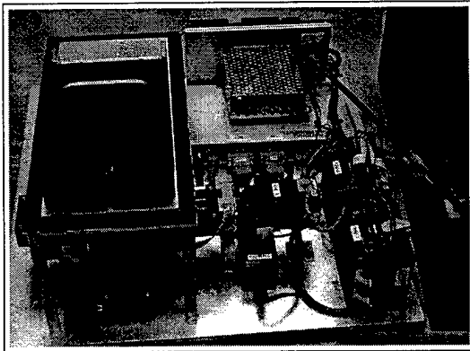
Fig. B-9 (a) The photo shows the MSI-ATP-Glow readout optoelectronics and mechanical components. (b) The exterior view of the prototype. The system will be further miniaturized in Phase II.
