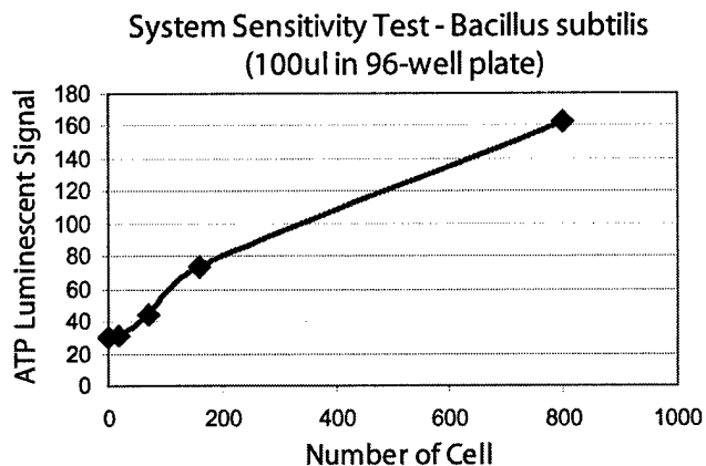
Fig. B-10. The Bacillus subtilis ATP luminescent signal measured by MSI-ATP-Glow prototype vs. the corresponding cell counts in culture samples. The number of colonies forming units per well was determined by live culture on nutrient agar plates.
