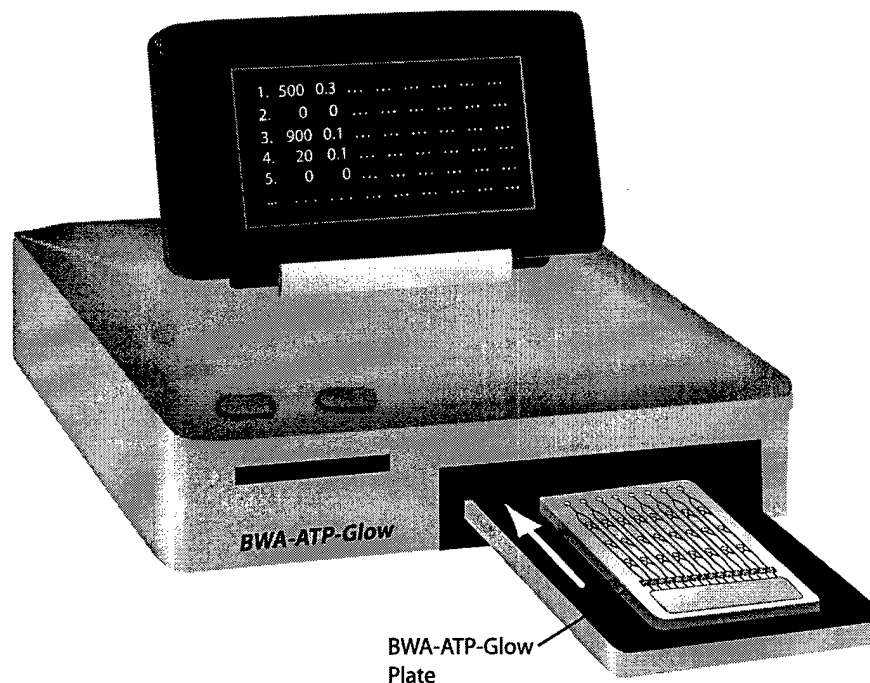
Fig. B-2. The figure shows the MSI's ATP-Glow portable system (11"x8"x4") including a disposable microplates (similar to 96/386 well format) for rapid, and high throughput evaluation of decontamination efficacy for an array of samples. In Phase II, the system will be miniaturized and automated to simplify operational procedure to a single step . The ATP-Glow microplate will be fabricated with patterned microchannels and microwells (50 \mu l - 200 \mu l) on a plastic cartridge. The system uses microactuator to perform the total automated the procedure and quantify the viable organisms remaining after treatment. (See Sec. B.3.5.1 and D.5 for details)
