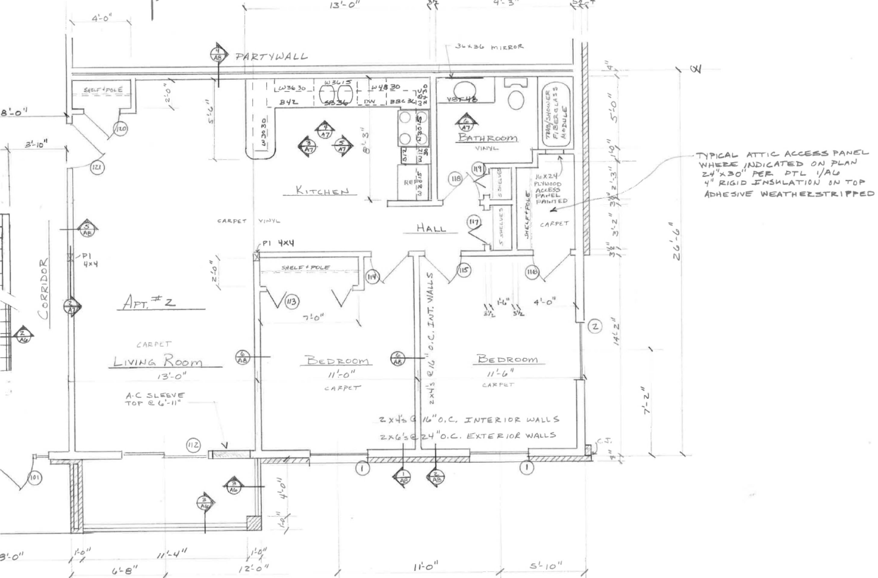
① TYPICAL APARTMENT PLAN 1/4" = 1'-0"
