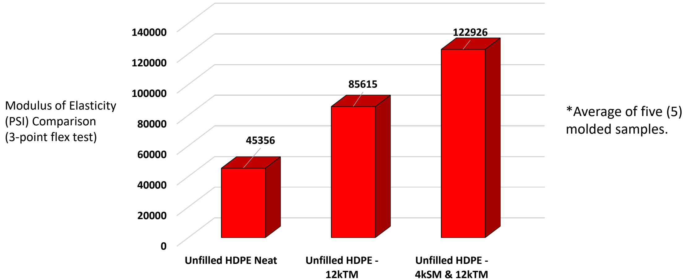
Compression Molded ICP 8"x18" Test Panels Modulus of Elasticity 3-Point Testing Rib Down
