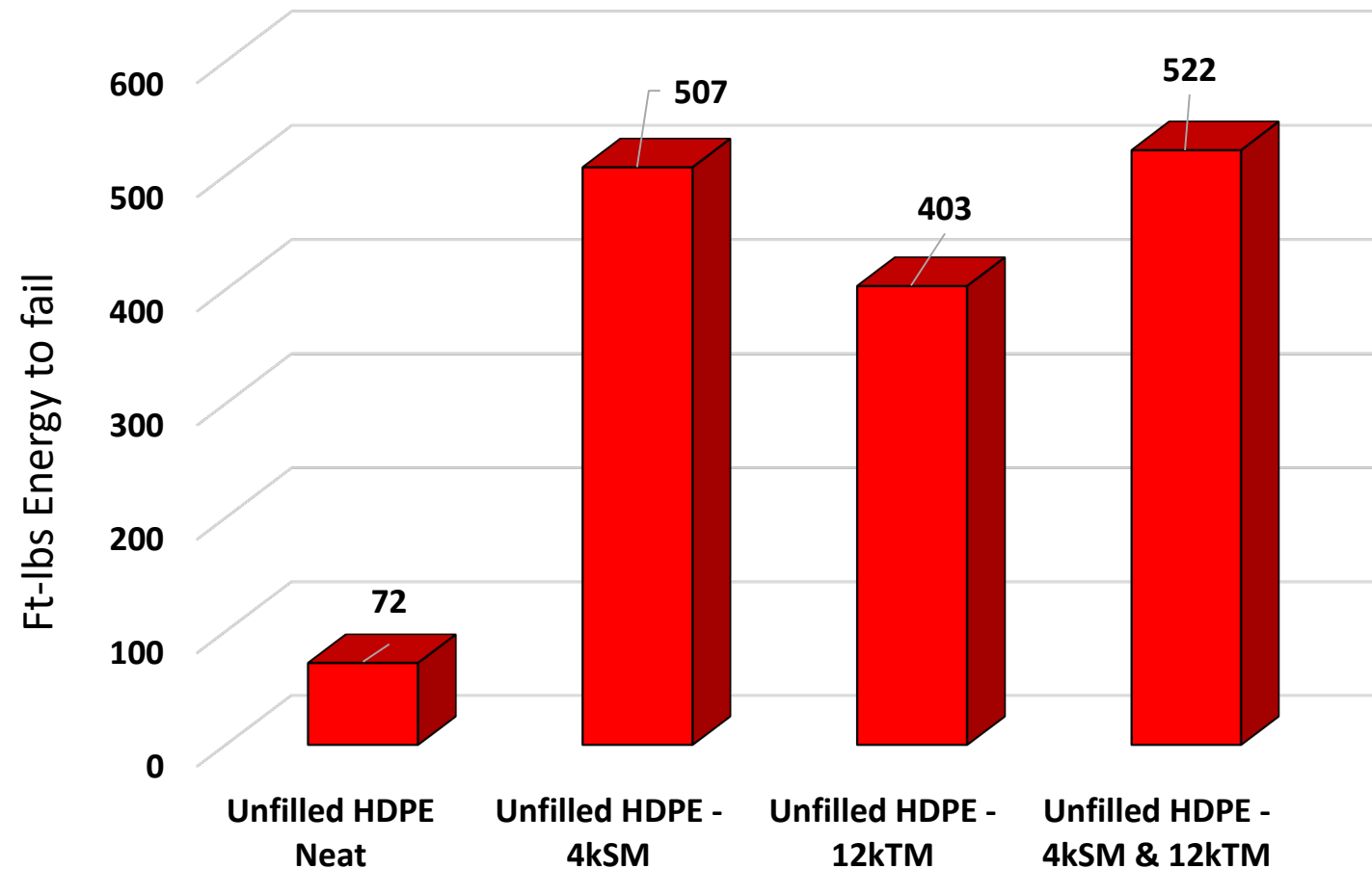
Compression Molded ICP 8"x18" Test Panels Impact Data - Pendulum Tester - RIB OUT
