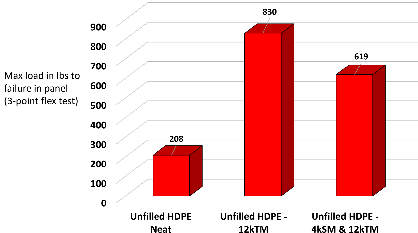
Compression Molded ICP 8"x18" Test Panels Overall Strength 3-Point Flex Testing Rib Down
