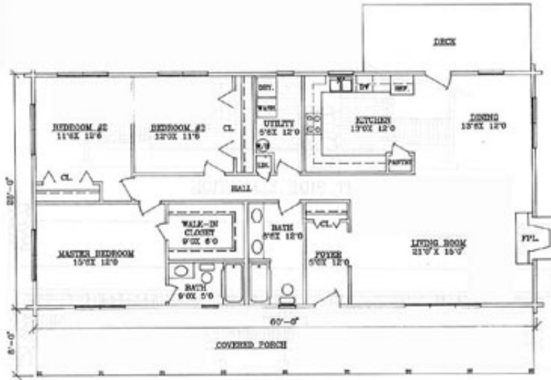
FLOOR PLAN
