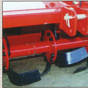
Durable rotor with four blades per flange.
