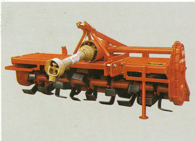
Rotor with 6 blades per flange. The standard version with universal blades.
