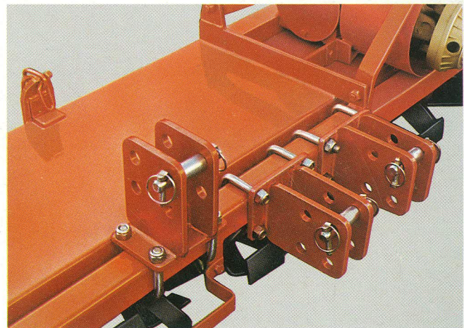
Three positions of the mounting plates to fit any tractor. They are adjustable on a square tube to obtain offsetable positions.
