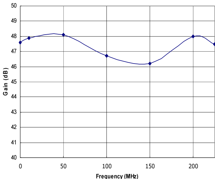
Figure 1: RFMS0.1-225-20 Typical Gain @ P_{out} = 20W .
