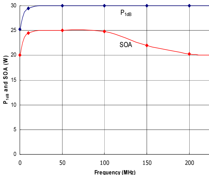
Figure 4: RFMS0.1-225-20 Typical P_{1dB} and Safe Operating Area (SOA). The amplifier is capable of delivering more power than it is safe to generate. Do not exceed the SOA without first contacting RFMPT to discuss your application.
