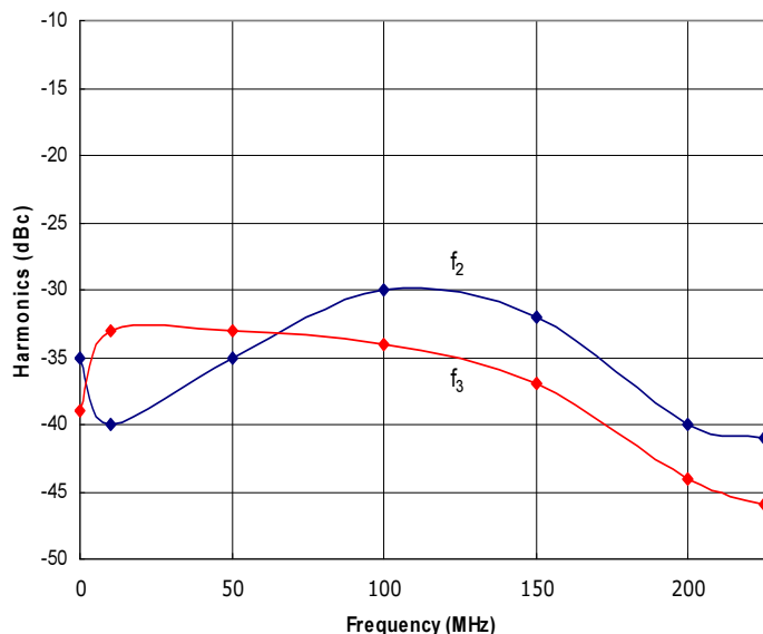
Figure 3: RFMS0.1-225-20 Typical f_2 and f_3 @ P_{out} = 20W .
