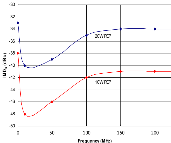
Figure 2: RFMS0.1-225-20 Typical IMD_3 , \Delta f=10kHz , @ P_{out} = 20W and 10W PEP.
